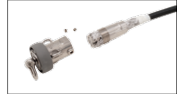
Pull the terminal over the line and fold the core of the line over the wedges. Insert the wedges to the terminal.
